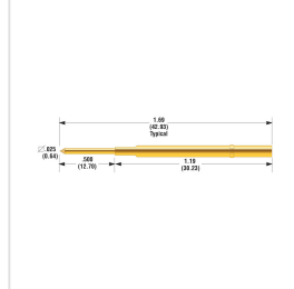
EPR-25W-2LL
