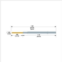
EPR-25W-2
