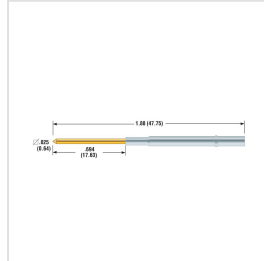
EPR-25W-2L
