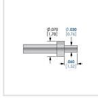
STP-25J140-3G
